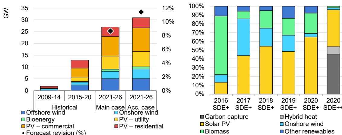
Figure 1.28 Netherlands renewable capacity additions, 2009-2026 (left) and share of budget award by technology, 2016-2020 (right)
