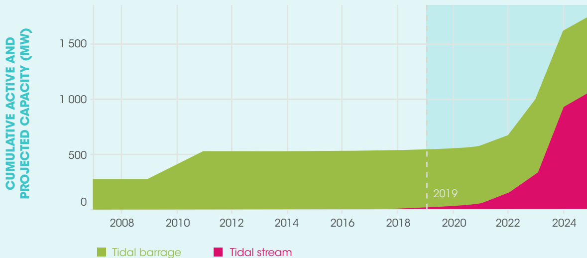
Figure 11: Active and projected cumulative tidal energy capacity
